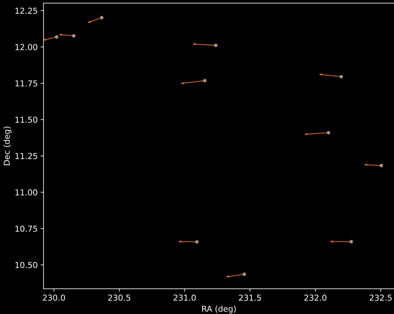
APOGEE DR17 Cluster 22 Proper Motion Vectors (n=11)
