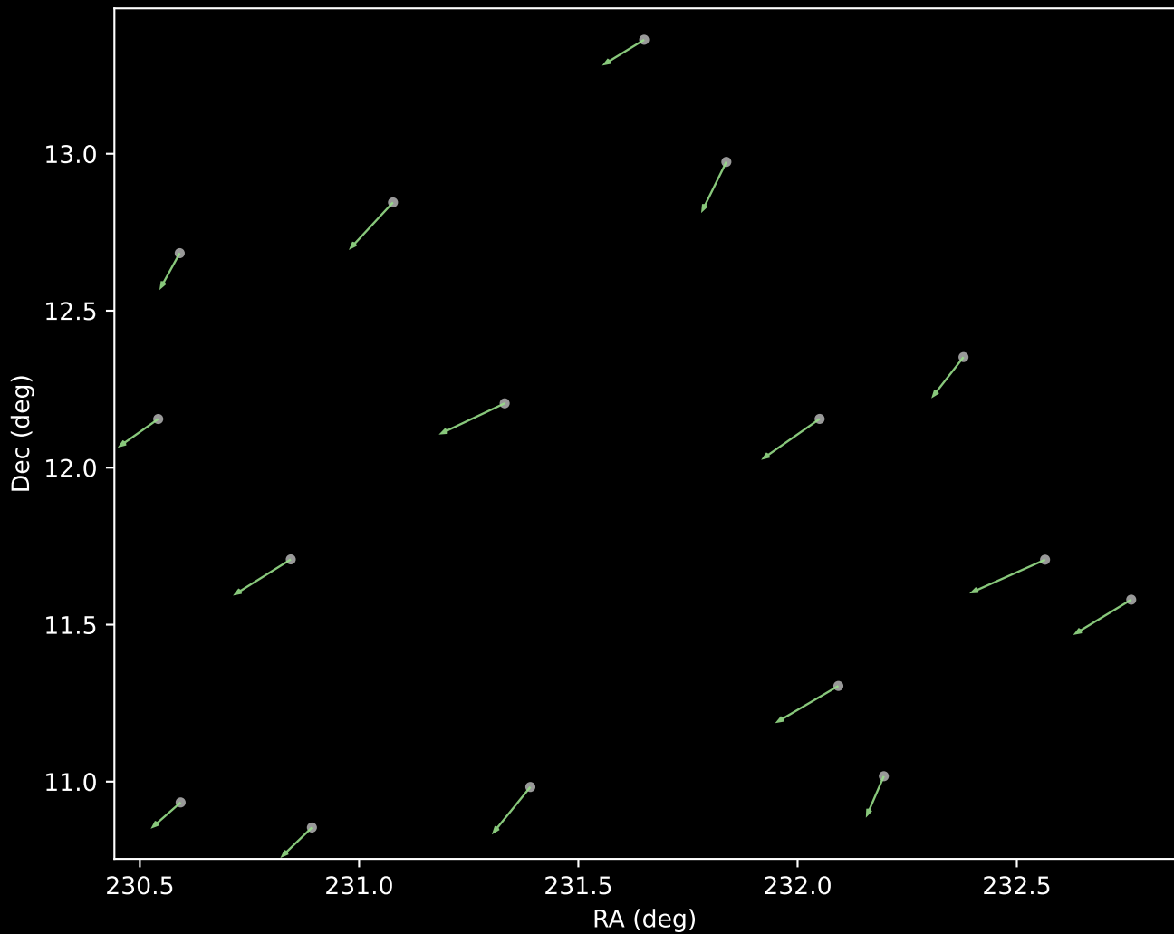
APOGEE DR17 Cluster 25 Proper Motion Vectors (n=16)
