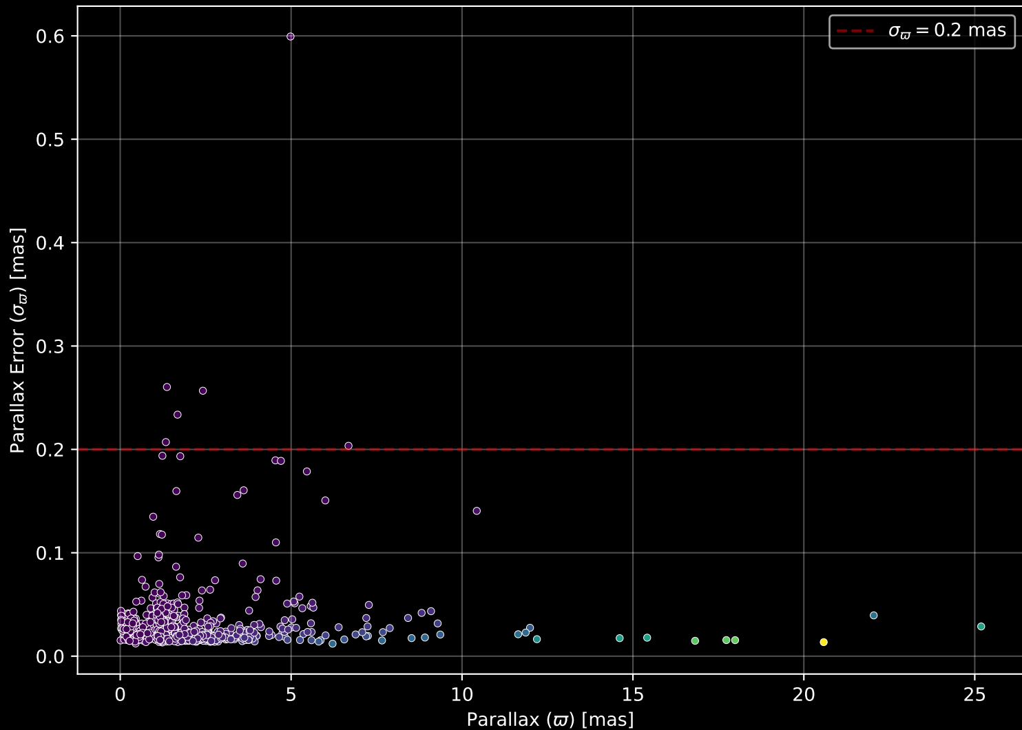
APOGEE DR17 Field: [GD1-2] Parallax Quality (n= 722)
