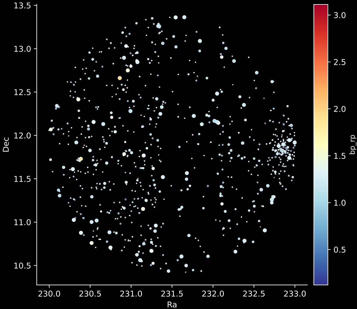
APOGEE DR17 Field: [GD1-2] Stars: 722
