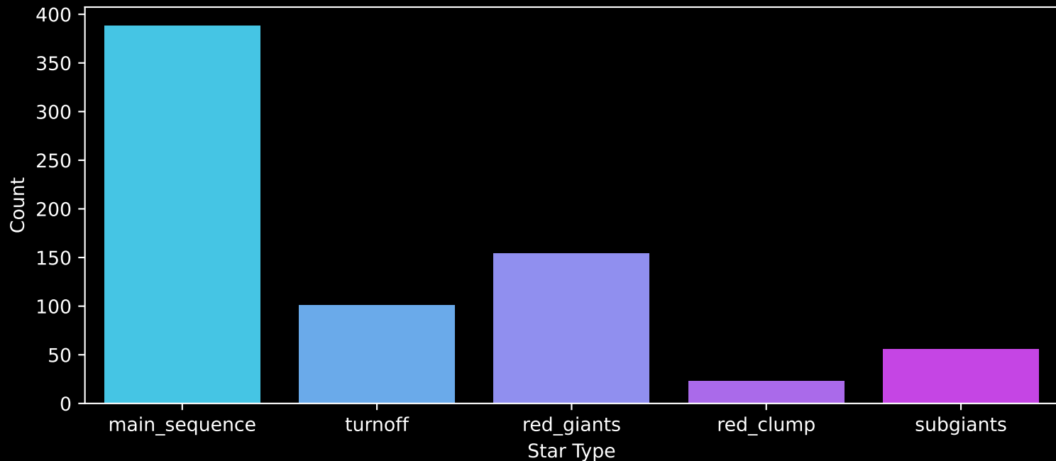
APOGEE DR17 Field: [GD1-2] Count plot of Star Type
