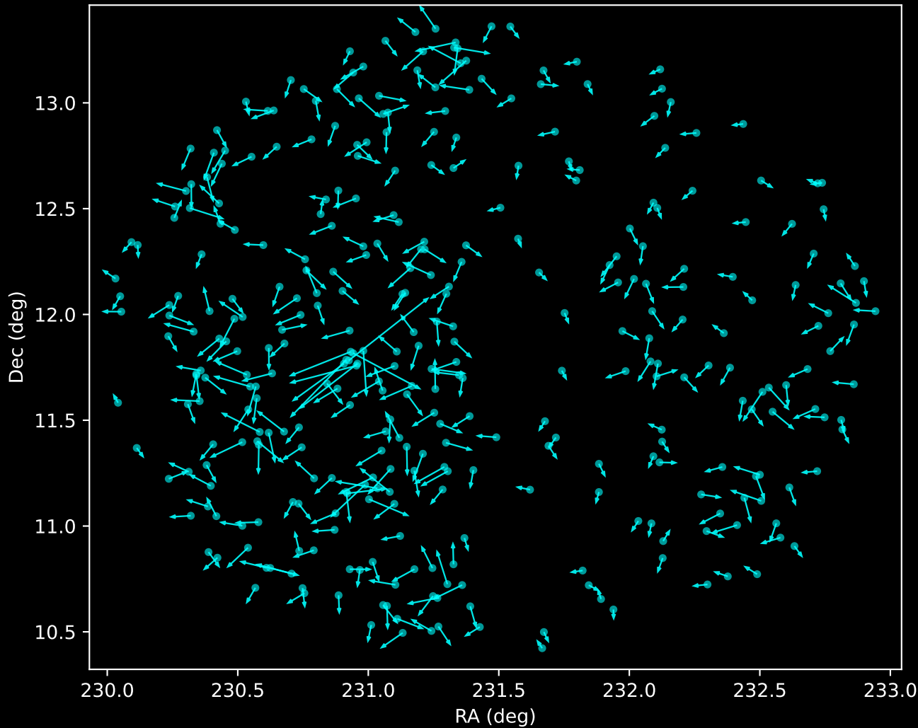
APOGEE DR17 Noise Stream Proper Motion Vectors (n=348)
