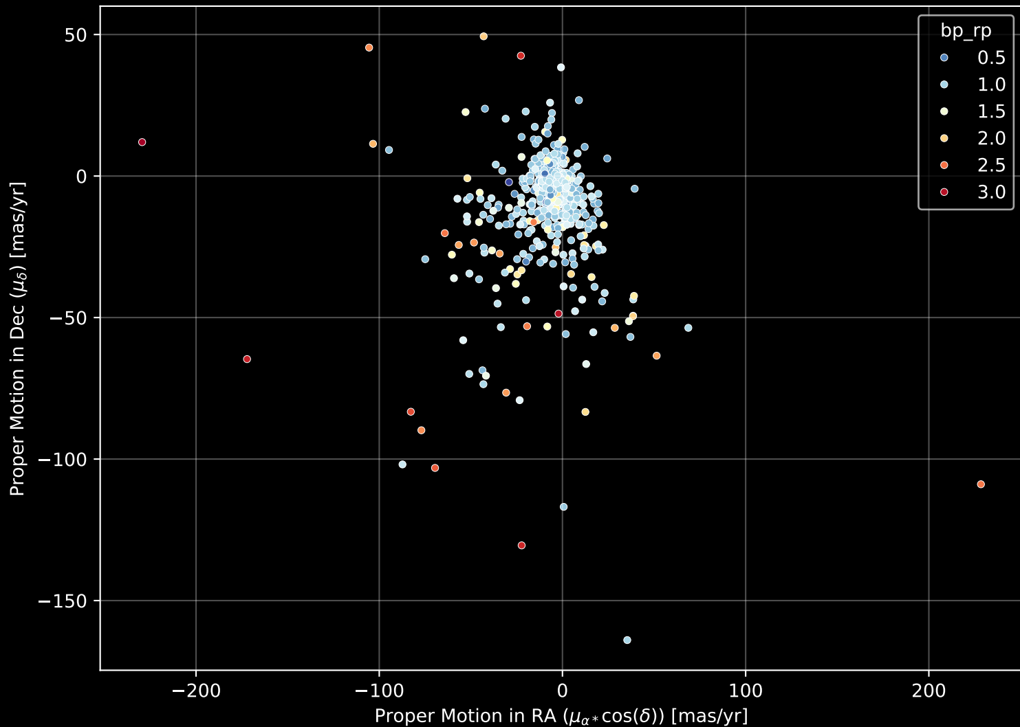
APOGEE DR17 Field: [GD1-2] Proper Motion Diagram (n= 722)
