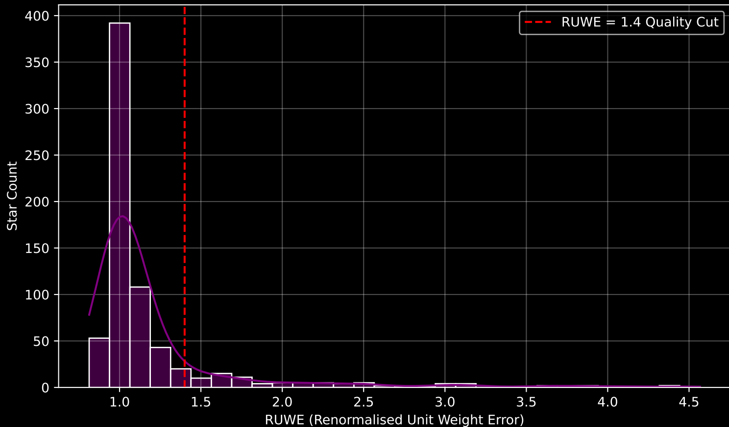
GAPOGEE DR17 Field [GD1-2] RUWE Distribution (n= 704)
