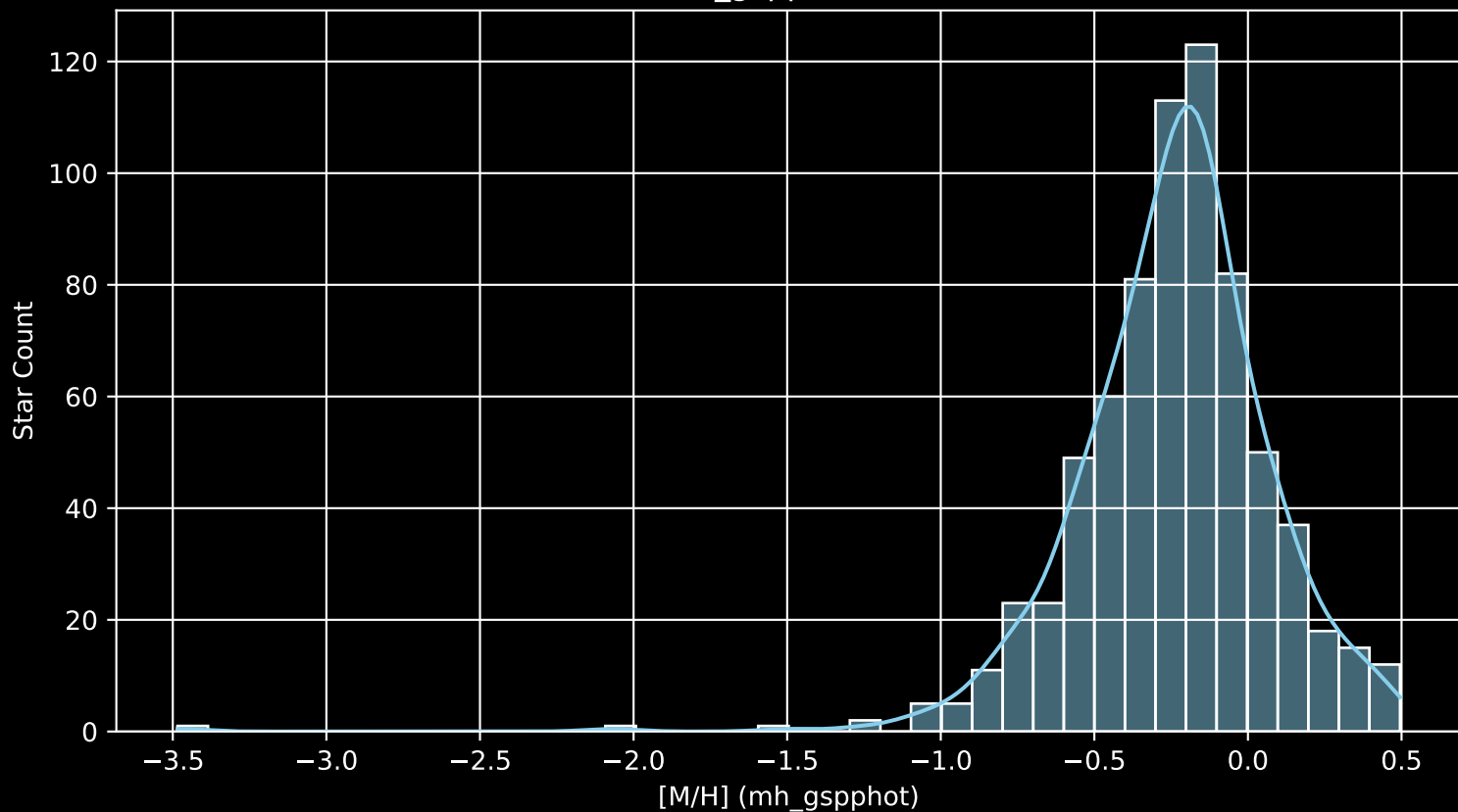
APOGEE DR17 Field: [GD1-2 [M/H] (mh_gspphot) (n= 712)
