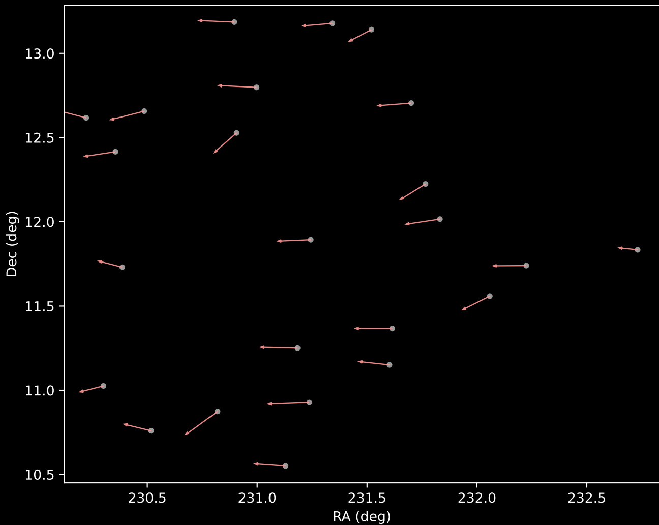
APOGEE DR17 Cluster 27 Proper Motion Vectors (n=24)
